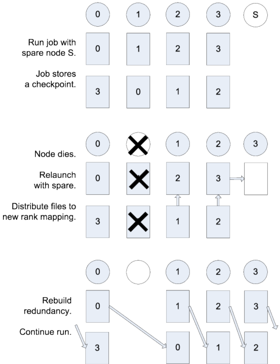
Fig. 2.2: Example restart after a failed node with Partner
