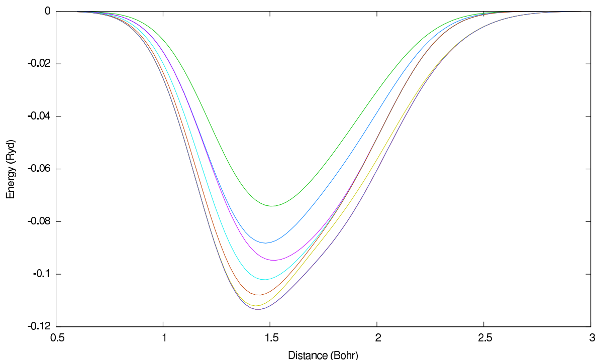
Figure 5: Free energy surface
