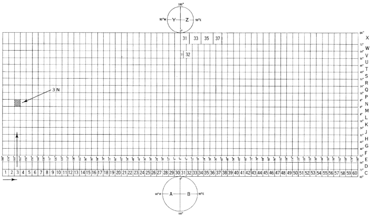
Figure A-9. MGRS Zones and Bands
